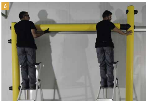
6 Position and fix horizontal beam to posts.
